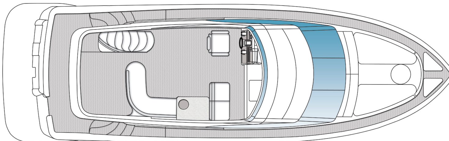
Standard Bridge (shown with pedestal helm seat)
